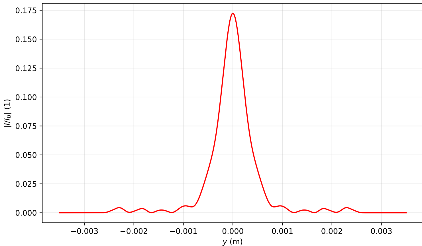
Intensity profile I(x=0, y, z=3.184)/I_0 , \text{Pin}=6.0\text{Pcr} , artificial time
